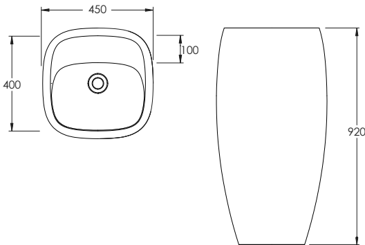
33150101 LAVABO FREE STANDING NUR PLAN Lavabo freestanding Nur con piano rubinetto Washbasin freestanding Nur with tap plan
