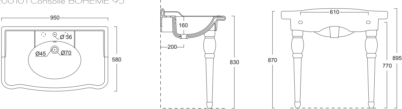
28260101 Consolle BOHEME 95 28260101 Consolle BOHEME 95
