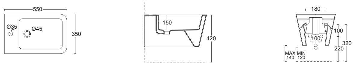
31220101 Bidet sospeso HIDE SQUARE 31220101 Wall hung bidet HIDE SQUARE
