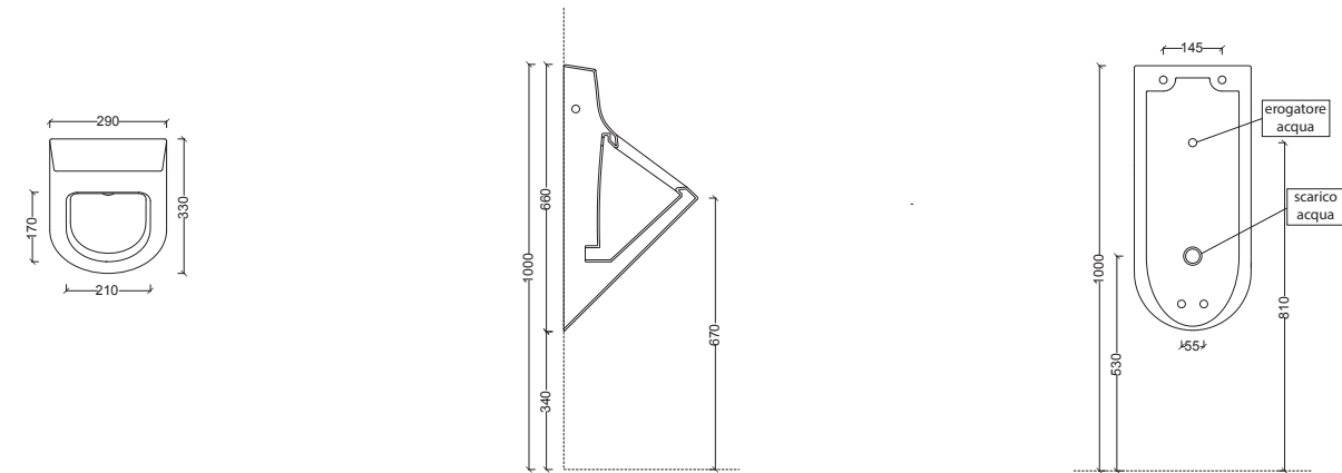
22260101 Orinatoio FORM
